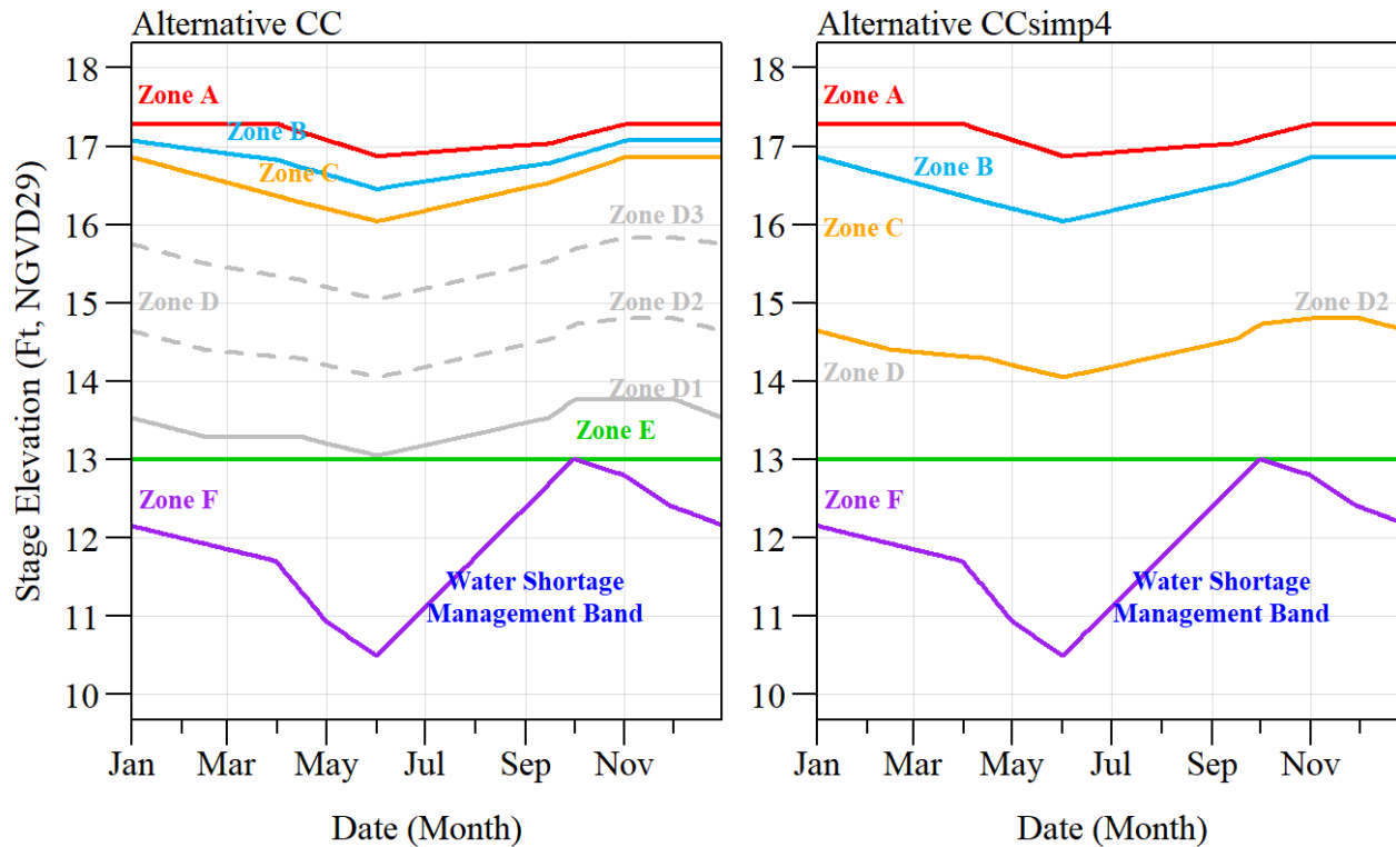
CC and 'CCsimp4' simplified regulation schedule.
