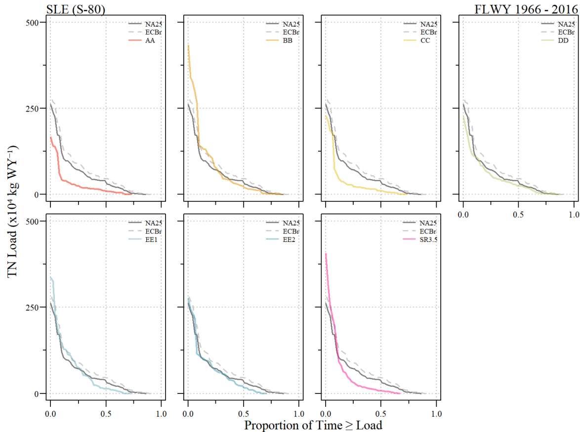
Cumulative distribution/load duration curve comparison of S-80 TN loads for each alternative relative to FWO (NA25) and ECB (ECBr).
